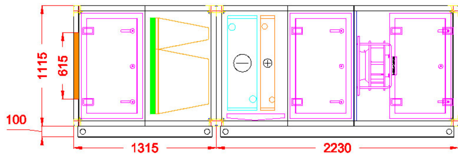
Right View
