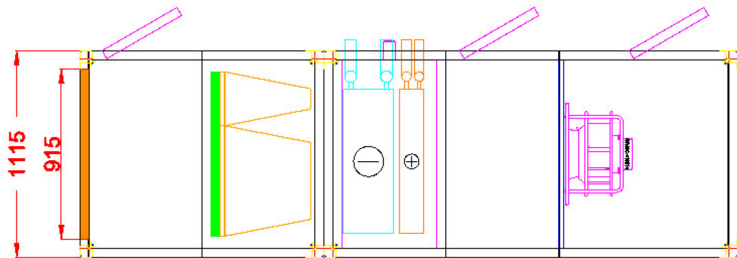
Top View
